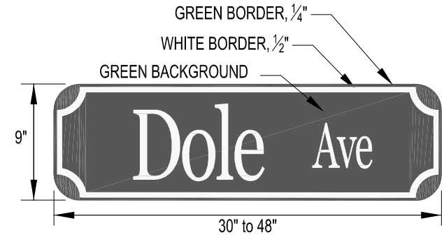
LOWER SIGN DETAIL
