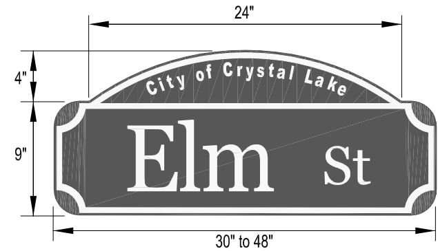
UPPER SIGN DETAIL
