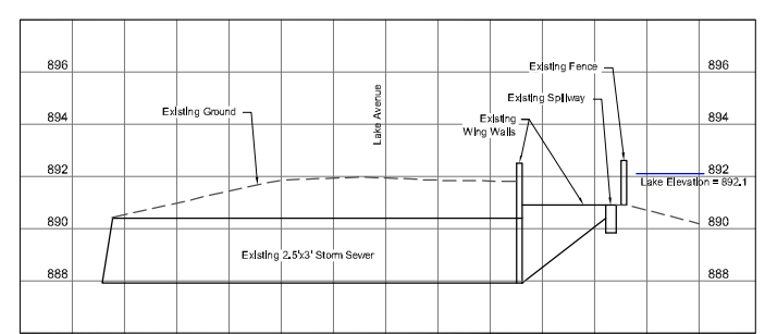
Spillway Cross Section Detail
