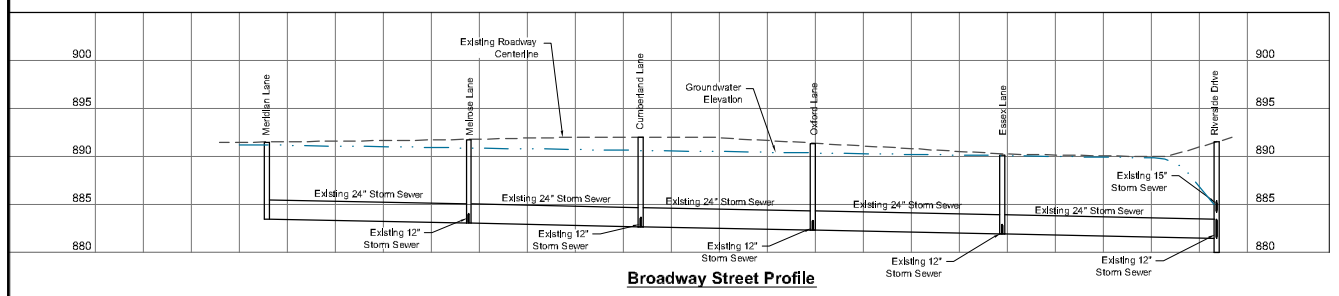
Broadway Street Profile
